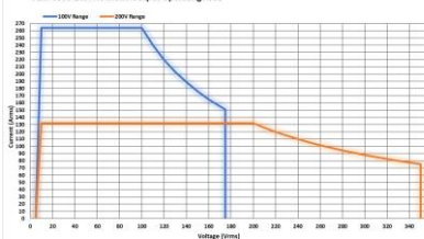
ASR-6600-26.4 AC Mode Output Operating Area
