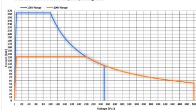
ASR-6600-26.4 DC Mode Output Operating Area
