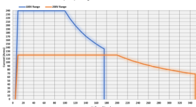
ASR-6600-24 AC Mode Output Operating Area
