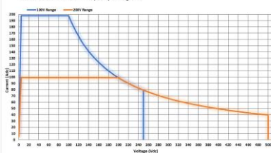
ASR-6660-19.8 DC Mode Output Operating Area
