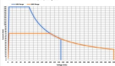
ASR-6500-15 DC Mode Output Operating Area
