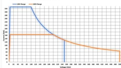
ASR-6600-33 DC Mode Output Operating Area
