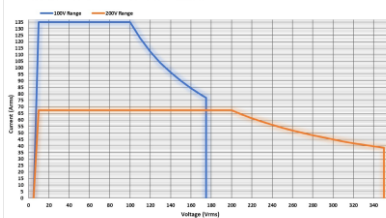
ASR-6450-13.5 AC Mode Output Operating Area
