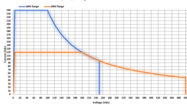
ASR-6600-24 DC Mode Output Operating Area
