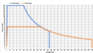
ASR-6450-13.5 DC Mode Output Operating Area
