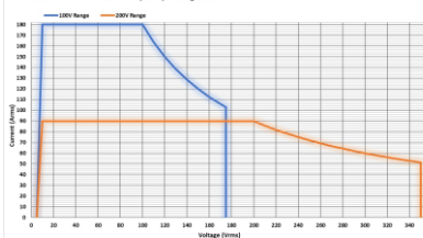
ASR-6600-18 AC Mode Output Operating Area
