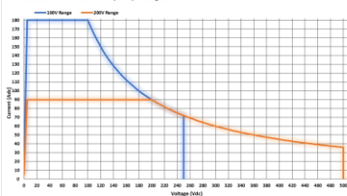
ASR-6600-18 DC Mode Output Operating Area
