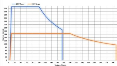
ASR-6600-33 AC Mode Output Operating Area
