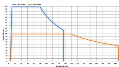
ASR-6660-19.8 AC Mode Output Operating Area
