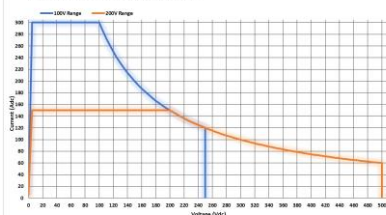
ASR-6600-30 DC Mode Output Operating Area
