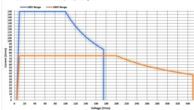
ASR-6500-15 AC Mode Output Operating Area
