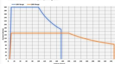
ASR-6600-30 AC Mode Output Operating Area
